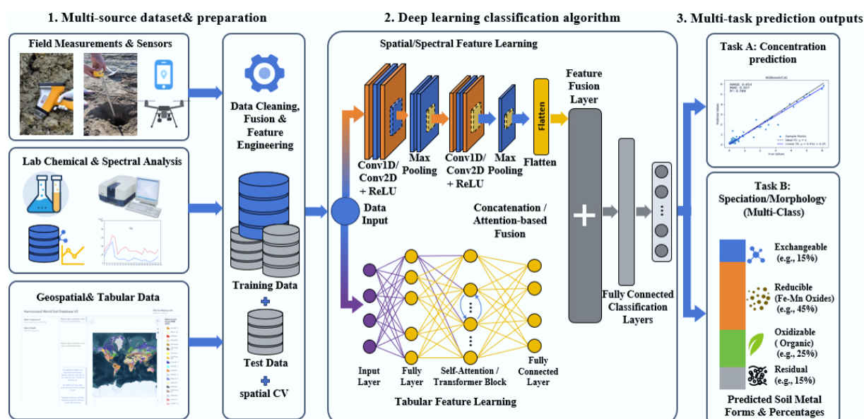
Fig. 2 AI-driven soil heavy metal prediction framework: from dataset to multi-task classification
