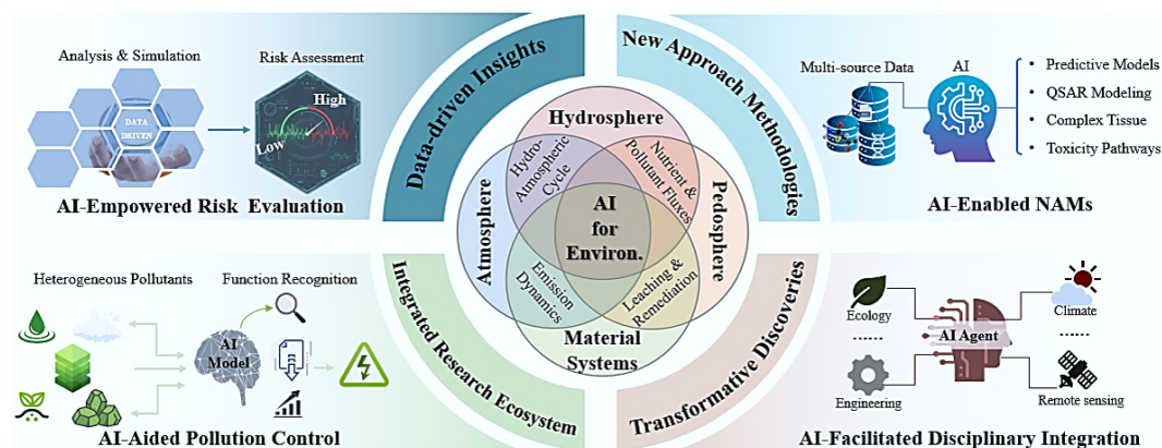
Fig. 1 AI for environment consists of four key areas, including data-driven insights, new approach methodologies, integrated research ecosystem and transformative discoveries.
