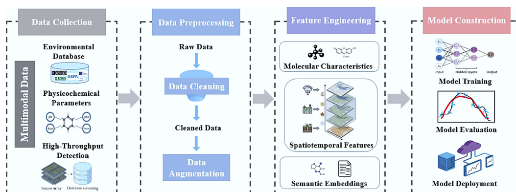
Fig. 3 Key components and workflow in environmental AI model development
